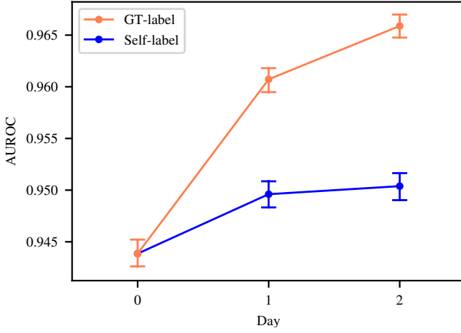
Fig. 8. Models’ performance over time: incrementally adding labeled data to the training set improves the AUROC (orange line) even using our self-labeling procedure (blue). Error bars denote 95% confidence intervals.
