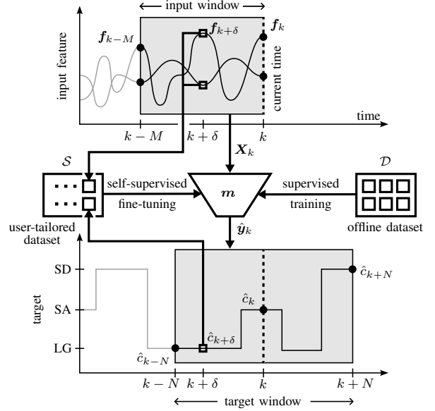
Fig. 2. Proposed approach: at each timestep k , the model \mathbf{m} is fed with an input window of the last M + 1 samples and outputs an estimate of walking modes in a target window including N timesteps ahead and behind; \delta marks the timestep in the target window where \mathbf{m} performs best. The estimate \hat{c}_{k+\delta} is used to pseudo-label the corresponding input \mathbf{f}_{k+\delta} and refine \mathbf{m} .
