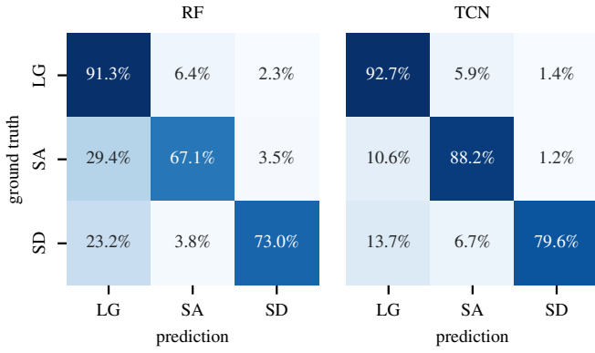
Fig. 5. Confusion matrix for the RF (left) and TCN approach (right).
