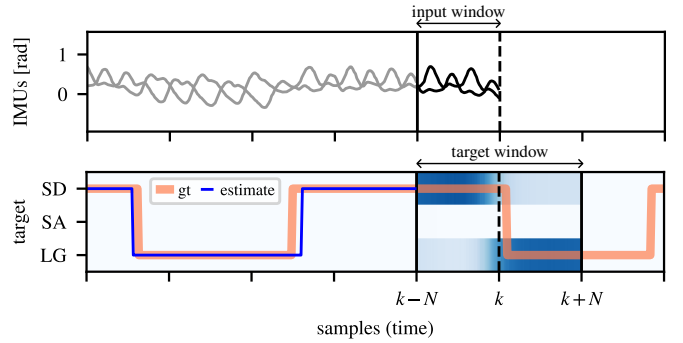
Fig. 7. TCN inference for a 14 s time-frame: IMUs signals composing the feature vector, with the input window (top plot, gray lines) and prediction of the model compared against the ground truth (bottom plot, blue and orange lines respectively). In the target window, the probabilities of each walking class are depicted with blue shades (the darker, the higher).
